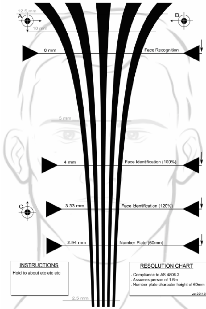
Figure E.5 CCTV Test Chart (DRAFT)
