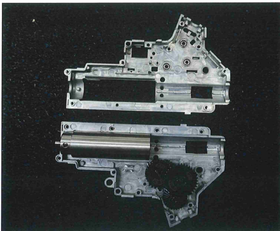
4.12 – Dynamic Tactical gear box housing Q0115360 with gears and piston sleeve from Q0116401.
