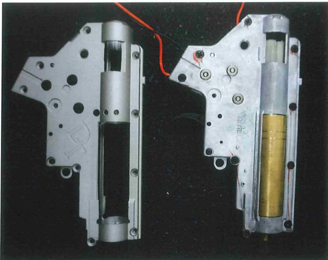
4.11 – Dynamic Tactical gear box housing Q0115360 on left and Lancer Tactical gear box on right.
