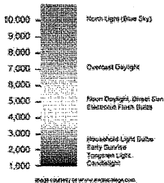
Colour Temperatures in the Kelvin Scale.
